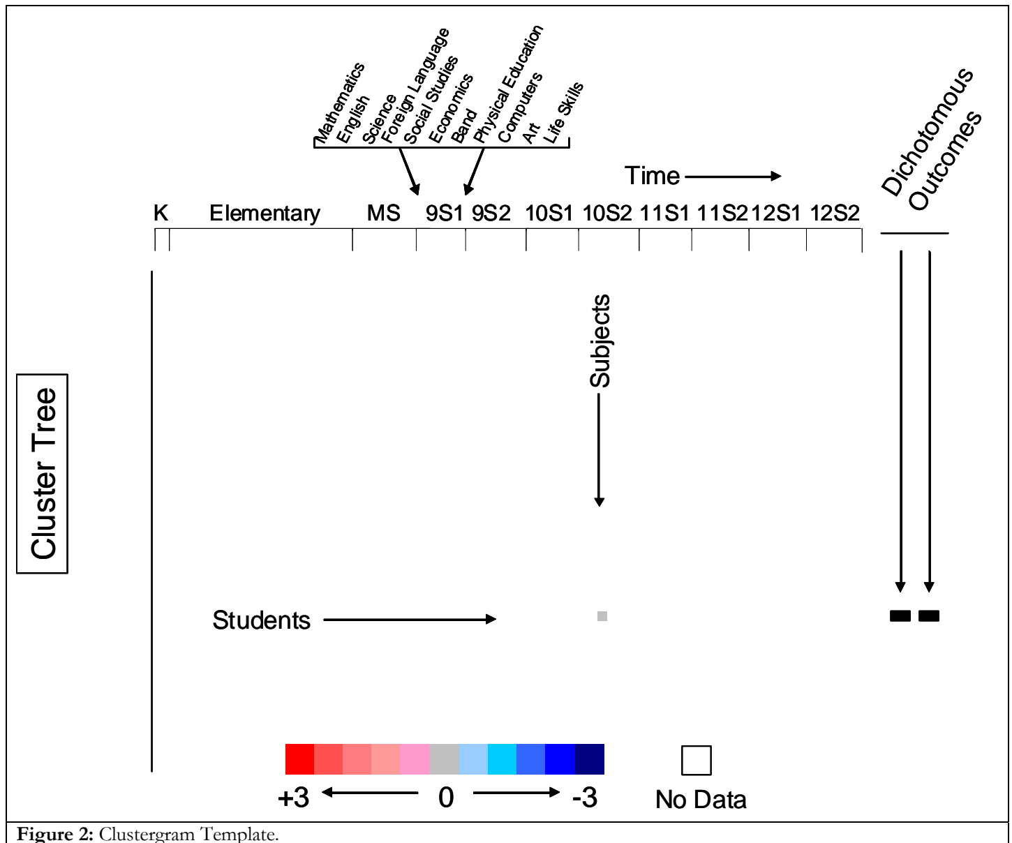
Figure 2: Clustergram Template.
