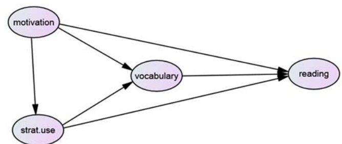
Figure 1. A hypothetical model of reading comprehension
