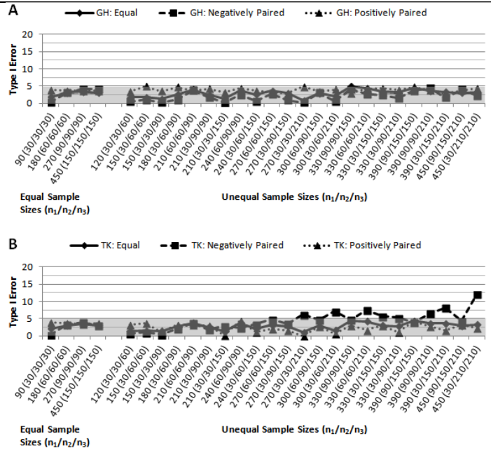
Figure 5. Type I error rate for declaring three populations equivalent under varying conditions of sample size and variability.
